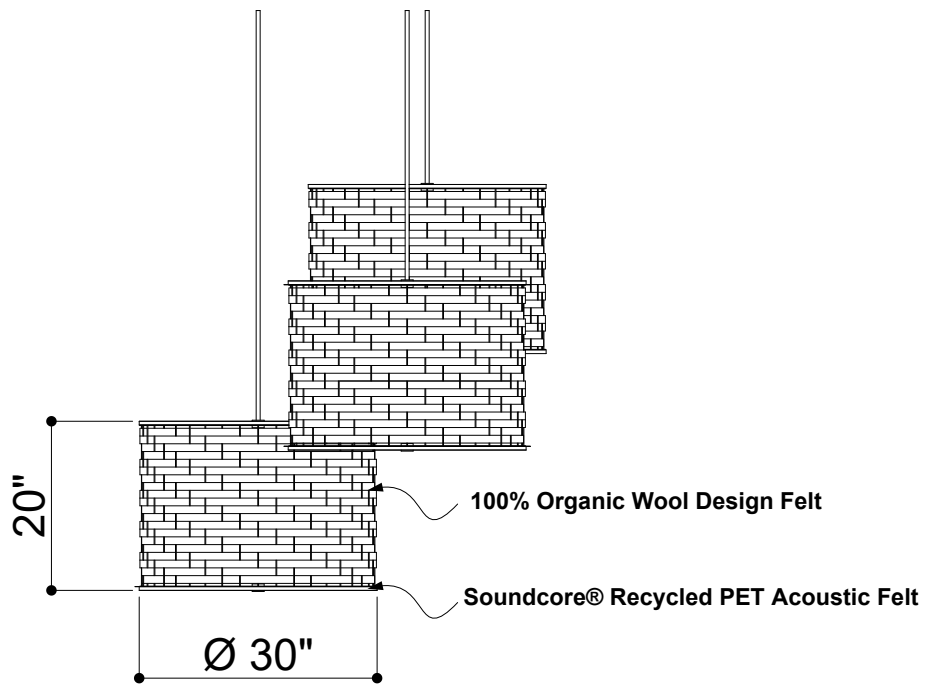
2 FRONT VIEW
