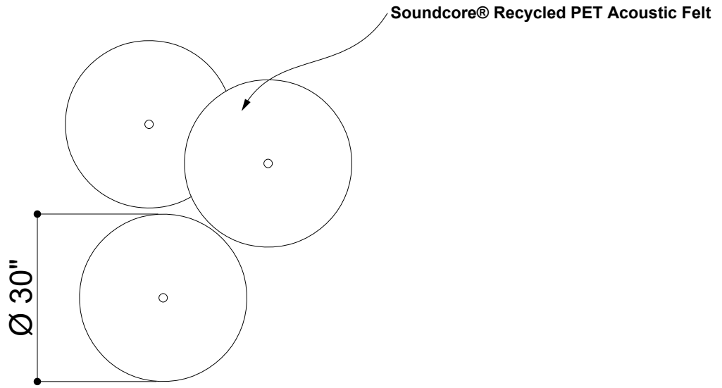
1 BOTTOM VIEW
